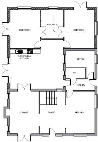
PROPOSED GROUND FLOOR PLAN 1-100 FIRST FLOOR UNAFFECTED BY PROPOSAL
