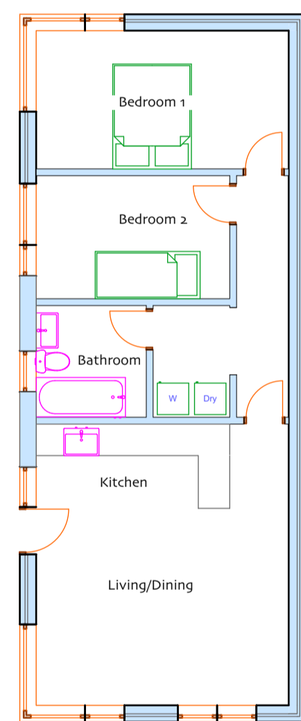
Proposed Floor Plan 1:100
